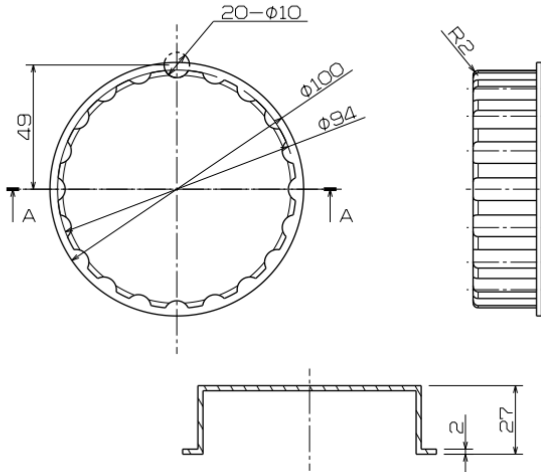
Section cut A-A
